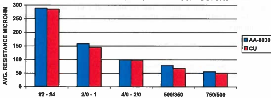
GRAPH 2: XHHW-2 (RW90-600V) AA-8030 & THHN-2 (T90) COPPER CONDUCTOR SIZES
