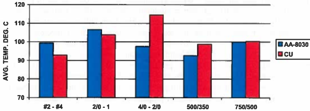
GRAPH 1: XHHW-2 (RW90-600V) AA-8030 & THHN-2 (T90) COPPER CONDUCTOR SIZES
