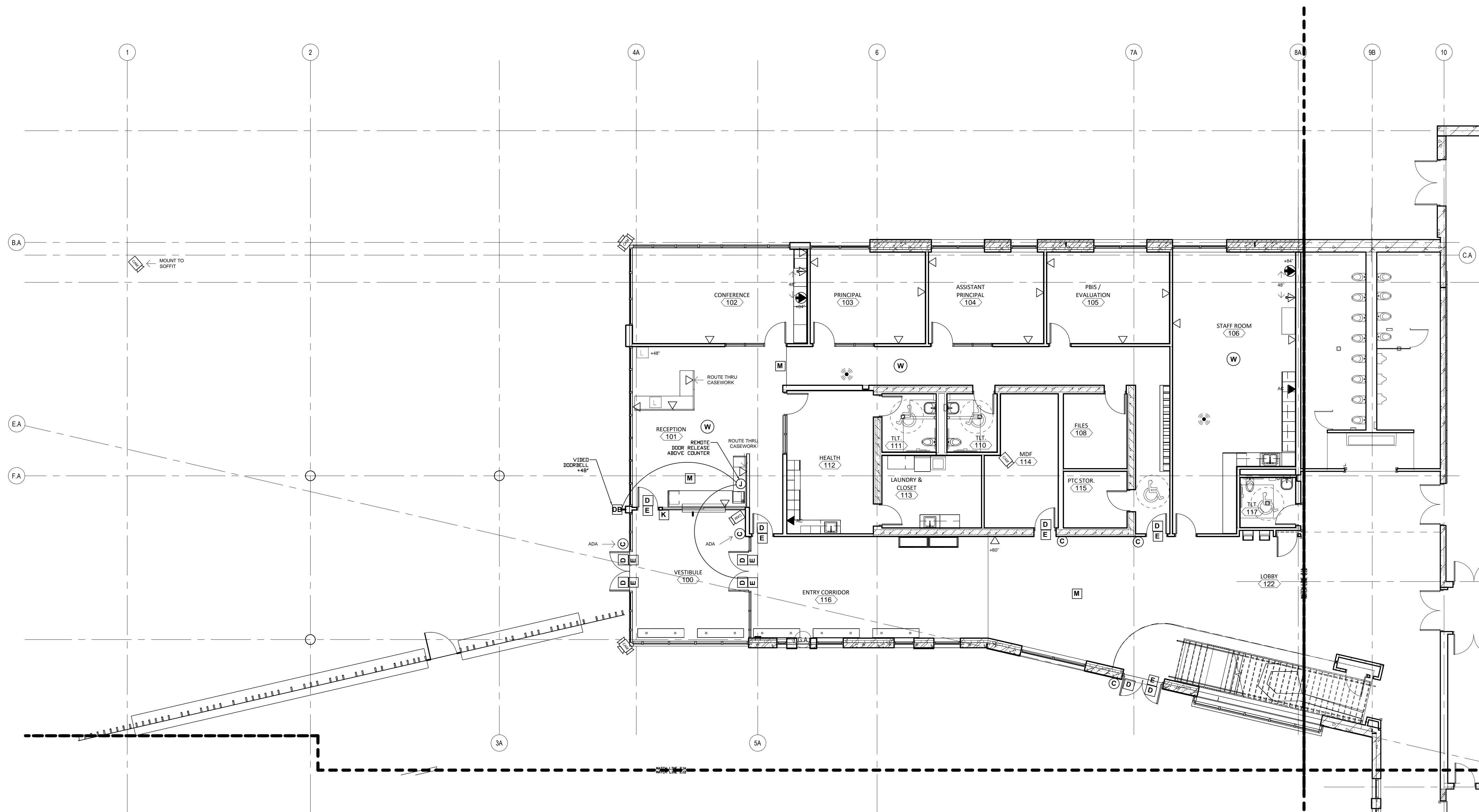
1 TELECOM PLAN, LEVEL 1 - AREA A 1/8" = 1'-0"
